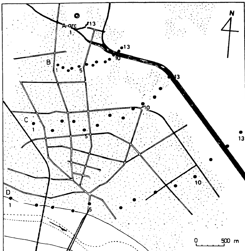
Fig 1. Sampling Points (1), (Arcs A,B,C,D). Dotted area shows the urban area.
