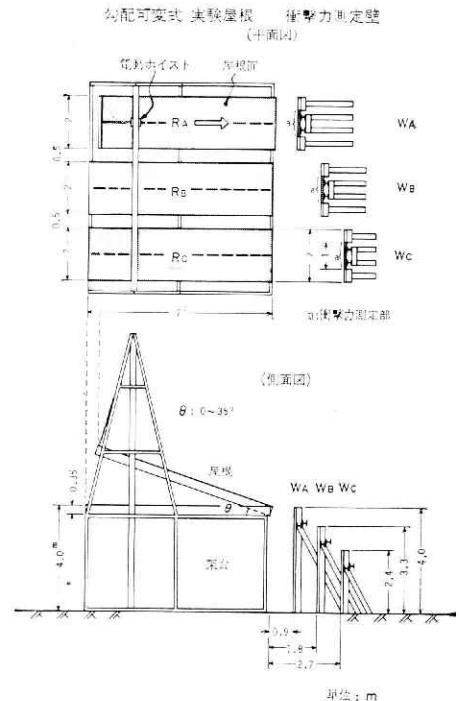
図 1 不均配可変式実験屋根及び衝撃力測定壁の配置図 Fig. 1 Plan and side view of experimental roofs and walls to measure the impact forces of snow blocks fallen from the roofs.
