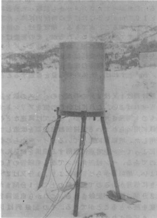
写真1 雪面に設置した降雪強度計の受雪部 Snow collecting instrument of snowfall intensity-meter being settled on the snow.
