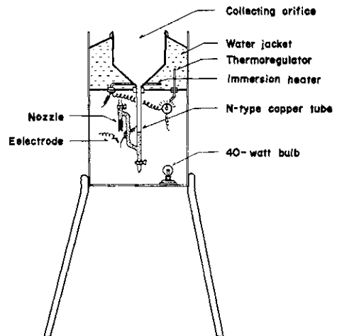
図2 受雪器の構造 Structure of the snow collecting instrument.
