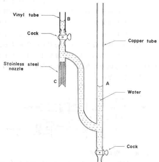
図3 N字管の構造 Structure of N-type copper tube.
