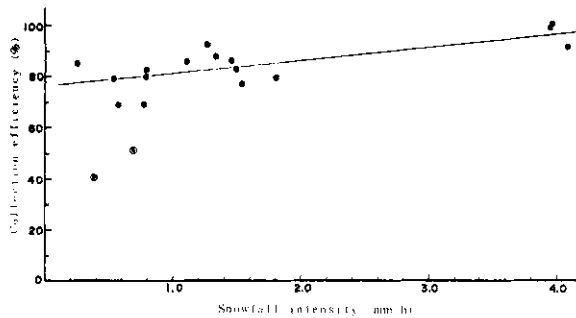
図9 捕捉率と降雪強度との関係 Relation between snowfall intensity and collection efficiency.
