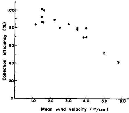
図8 平均風速と捕捉率との関係 Relation between mean wind velocity and collection efficiency.
