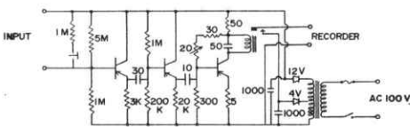
図4 増幅回路図 Schematic diagram of amplification circuit.
