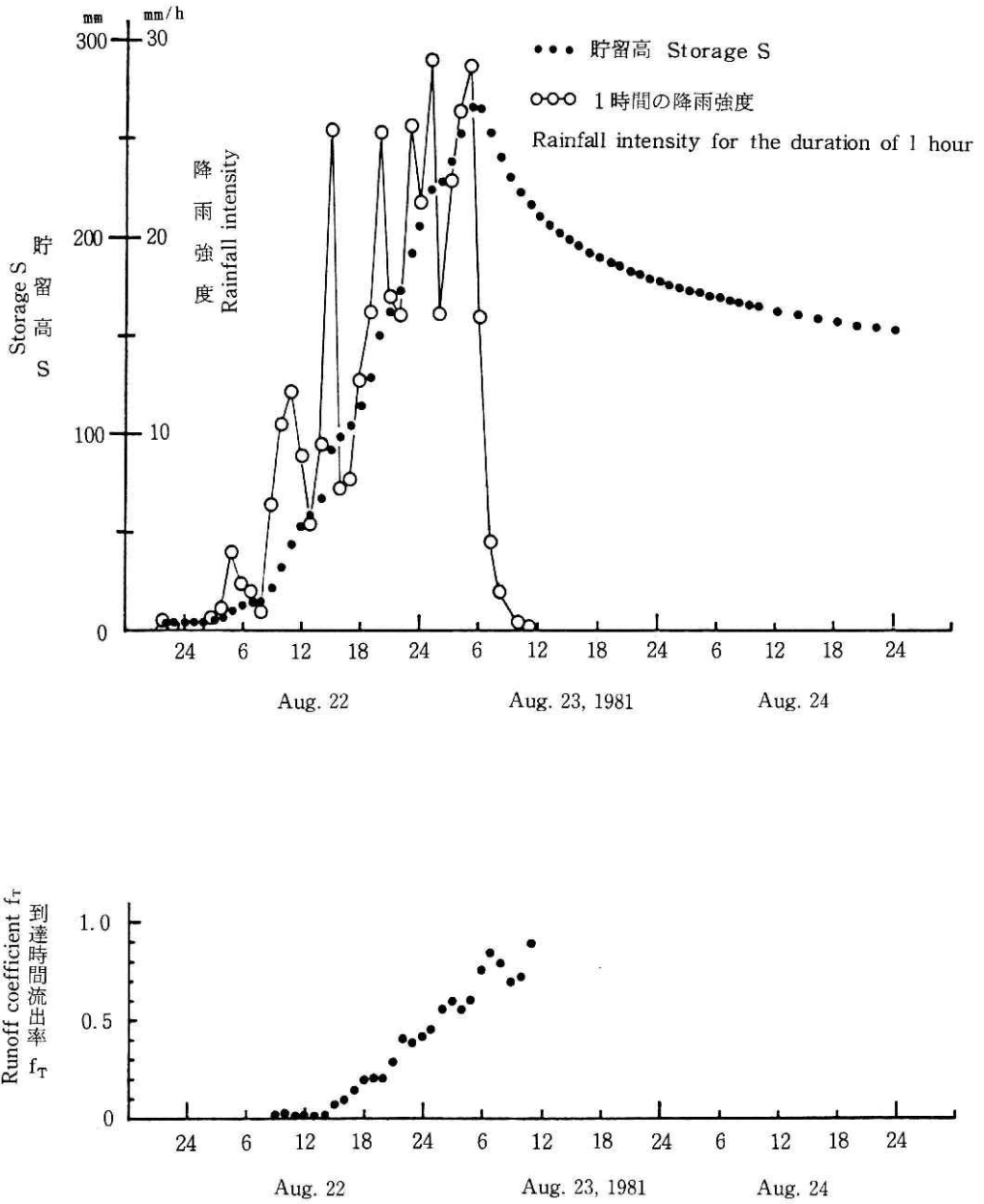
図3 C流域における到達時間流出率 f_r と貯留高 S の時間変化。 Fig. 3 Rainfall intensity, storage S of the rain water and runoff coefficient f_r in the C basin during the storm of August 23, 1981 are plotted on the same time axis for mutual comparison.
