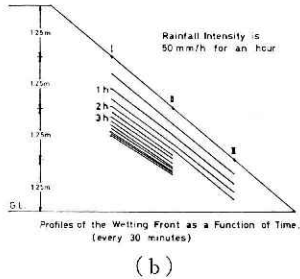
図5 浸潤面の下降状況および断面図 Fig. 5 Downward Movement of Wetting Front. & Profiles of the Wetting Front as a Function of Time.
